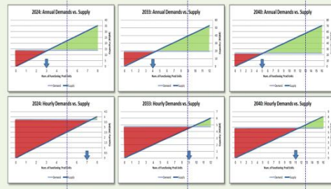
Fig. 3 – Annually & Hourly reliability of supply
